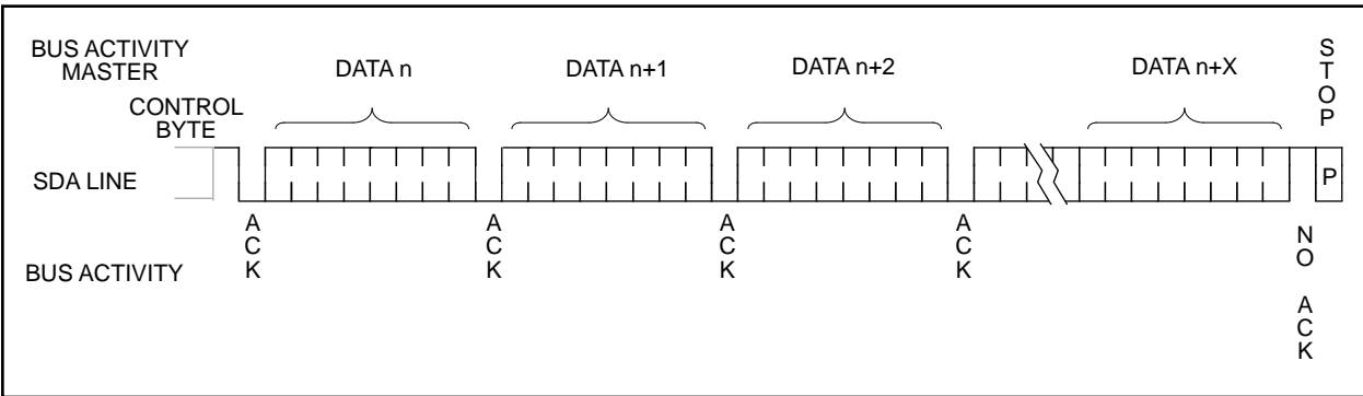
FIGURE 8-1: SEQUENTIAL READ
