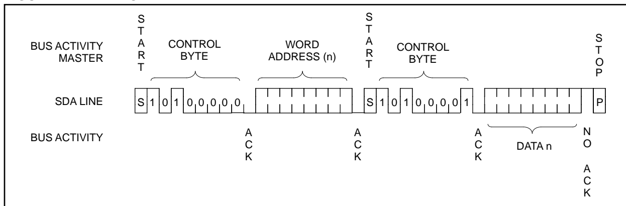
FIGURE 7-2: RANDOM READ
